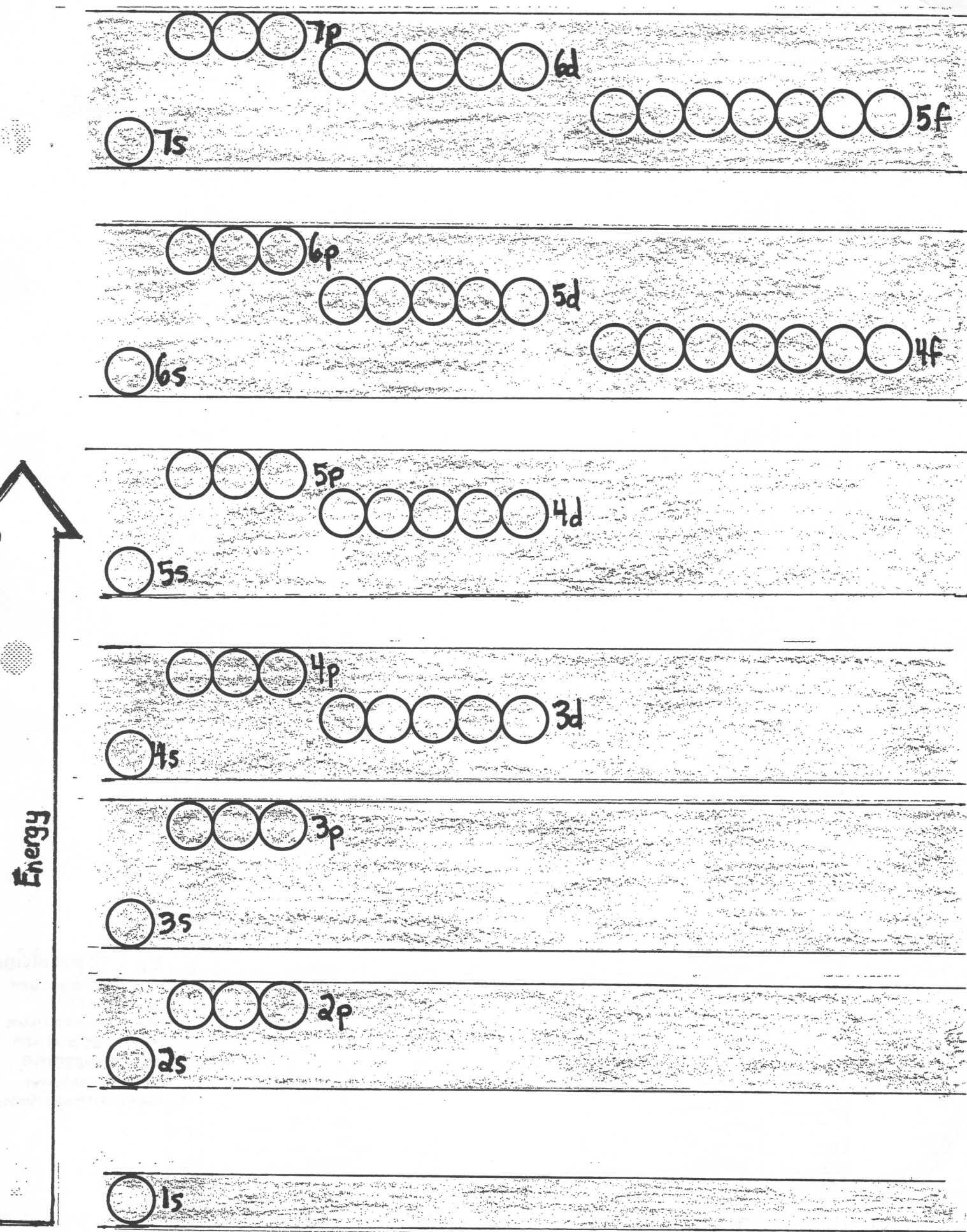
Energies of Electron Orbitals
